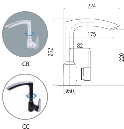
1/2" ZAMBEZI ZA007.5/7 ZA007.5/7CB ZA007.5/7CC
