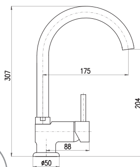
1/2" SEINA SE908.5/4 SE908.5/4CMAT
